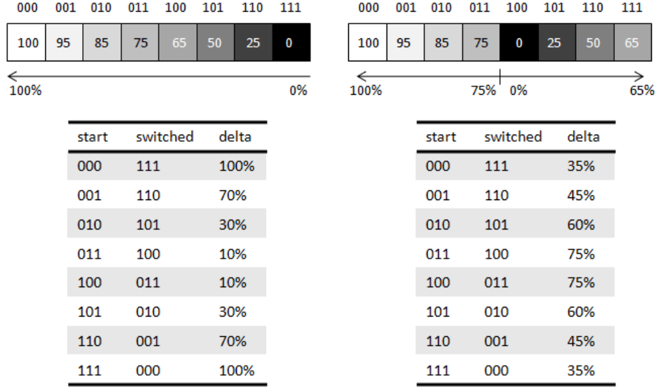
Fig. 8. Color palette organization for data masking.
